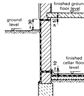
⑧ Damp-proofing of building with cellar; masonry walls on strip foundations
